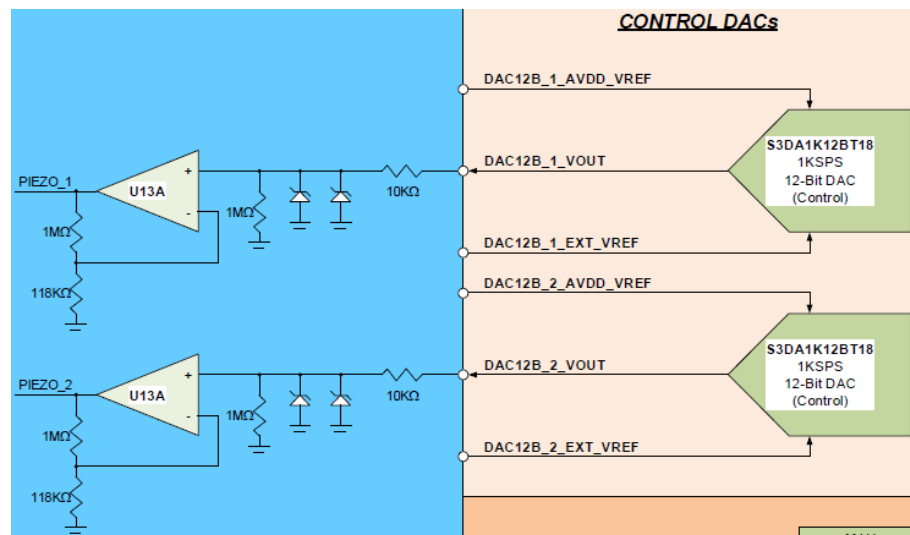
Figure 4: Dual channel drive consisting of 12-bit control DACs and PGAs
