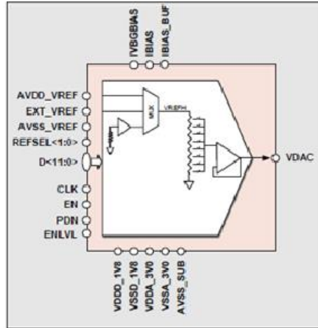
Figure 3: An example of a 12-bit control DAC IP block
