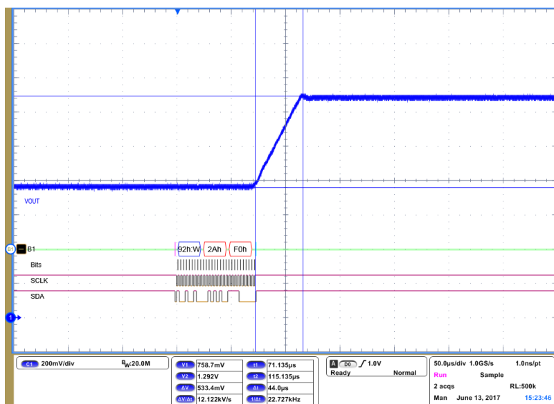
Figure 7: DVC step-up with 12.5mV/µS slew rate
