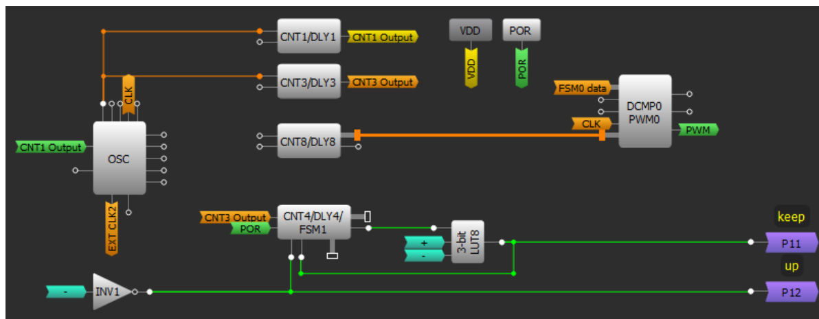
Figure 3: PWM Unit Design
